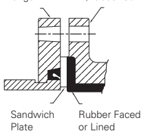
#7041 / #7043 Flange Flange to Mate (Rubber Surface)
