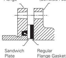
#7041 / #7043 Flange Flange to Mate (Serrated Face)
