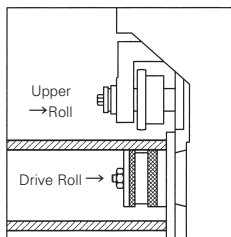
Pipe end is placed between the roll set (upper roll & drive roll)
