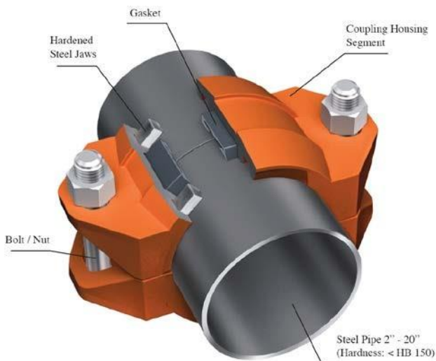
Model 79 Plain-End Coupling
