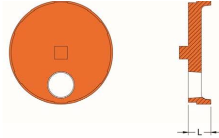
Model 7160T Transition Fitting
