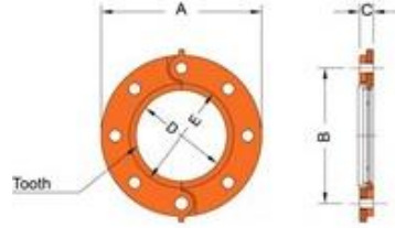
MODEL 7041 FLANGE ADAPTER - BS 10-E, 2" - 12"
