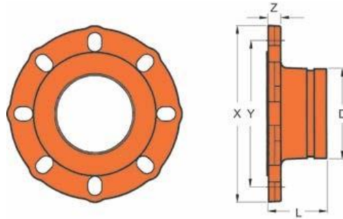
Model 7180 Universal Flange Adapter
