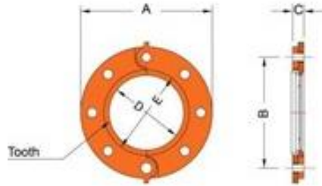
2"-12" (Hinged)
